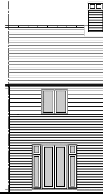
Rear Elevation
